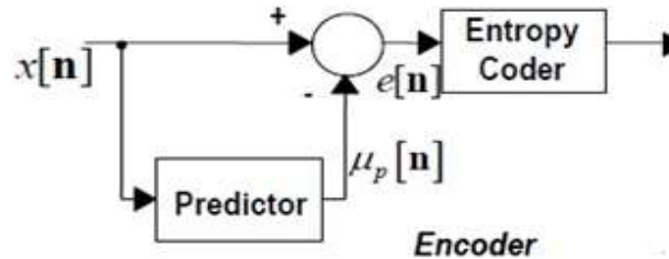
Fig 2. Lossless Predictive Encoder and Decoder
