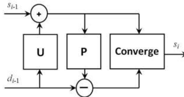
Fig.4. Reverse Lifting Scheme
